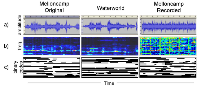
Figure 1: Representing audio. Three 10-second snippets of audio are shown: John Melloncamp original, Waterworld soundtrack, and John Melloncamp recorded. It is difficult to determine which snippet matches the song in the waveform audio representation (a). In the spectrogram images (b), certain similarities between the two Melloncamp snippets and distinguishing differences between the Melloncamp and Waterworld snippets become noticeable. Matching snippets are easily identified using our learned descriptions (c).
